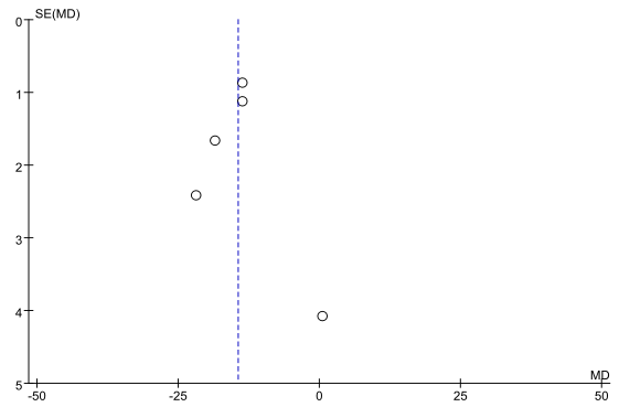
ROM of the knee joint postoperation at 6 months funnel plot
