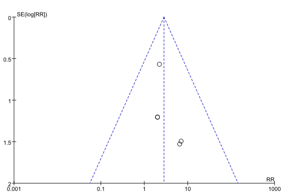
Malunion funnel plot
