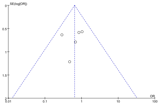
Overall excellent and good rates of knee functional funnel plot
