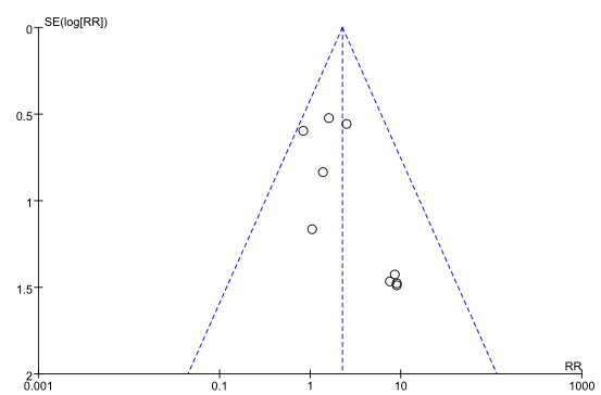
Overall complications funnel plot
