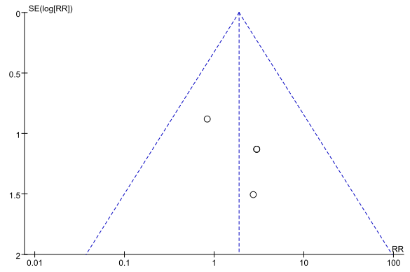
Delayed union funnel plot
