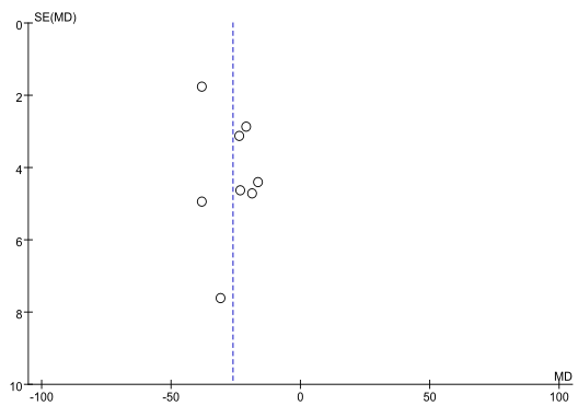
Operation time funnel plot
