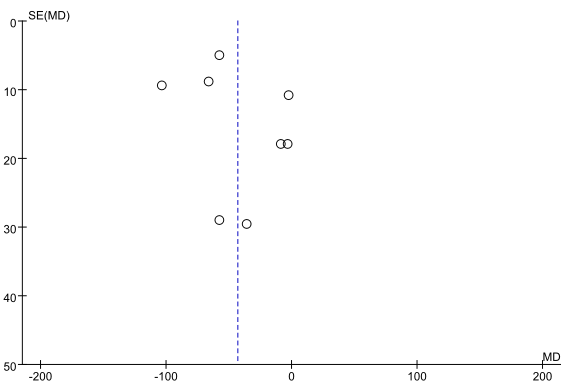
Intraoperative blood loss funnel plot
