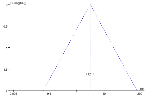
Plate fracture funnel plot
