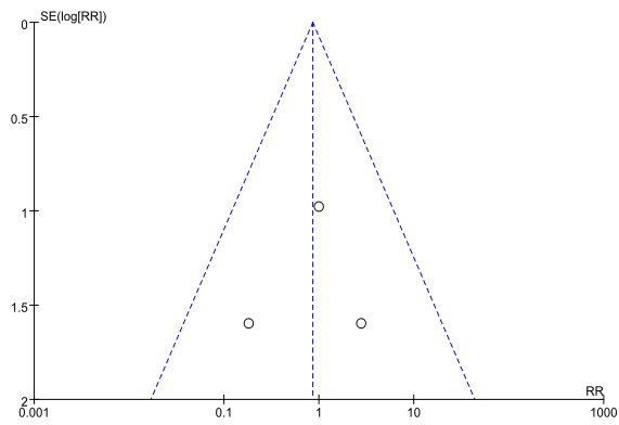
Incision infection funnel plot
