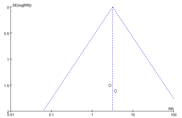
Nonunion funnel plot
