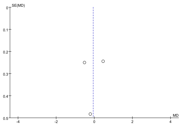
Fracture healing time funnel plot
