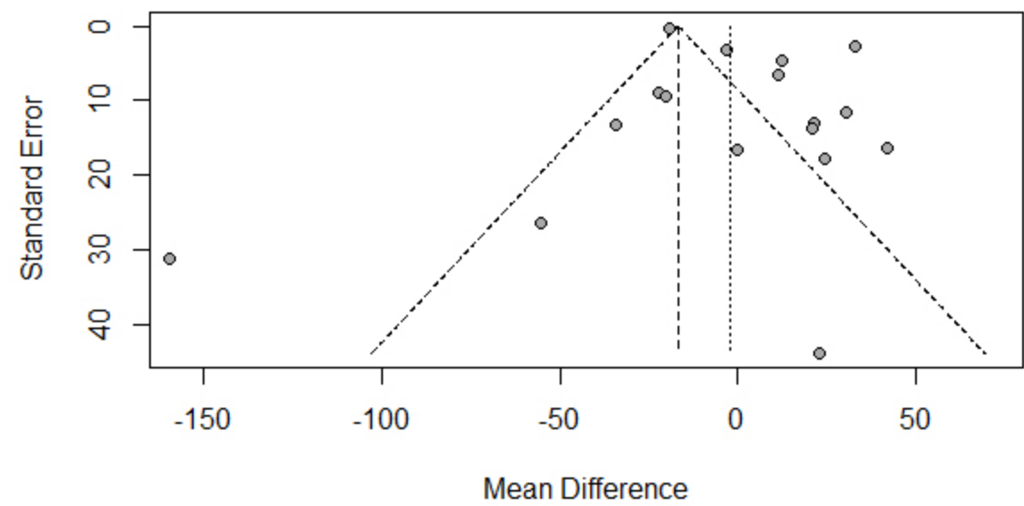
Operation time funnel plot
