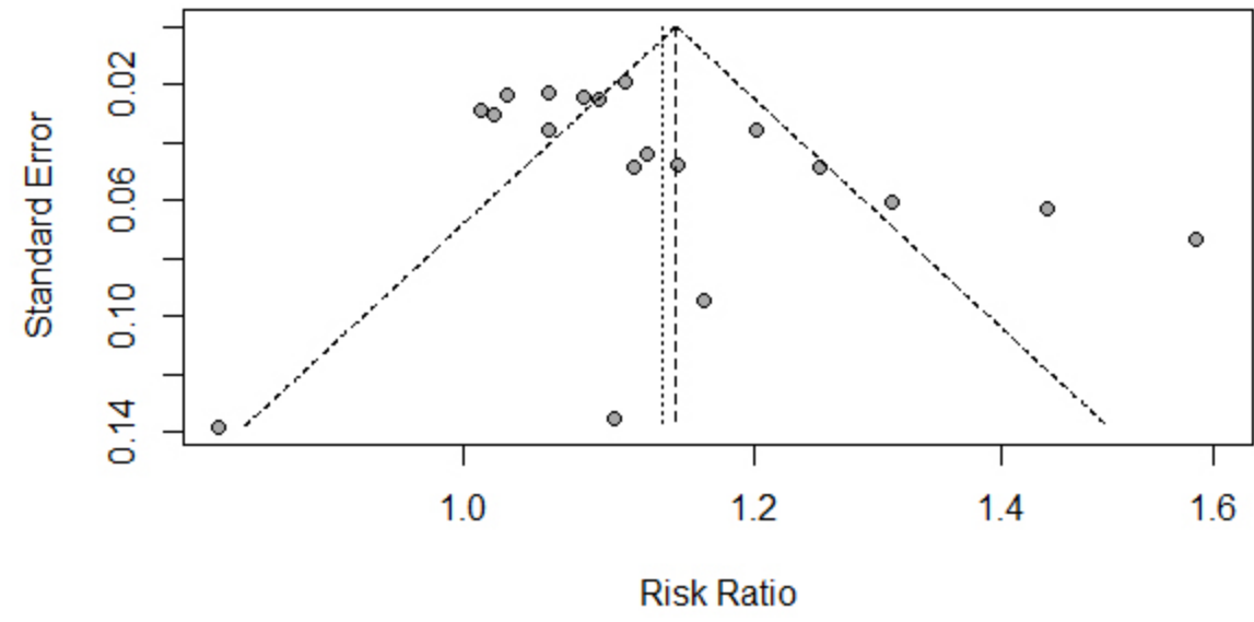
Screw position grade A funnel plot
