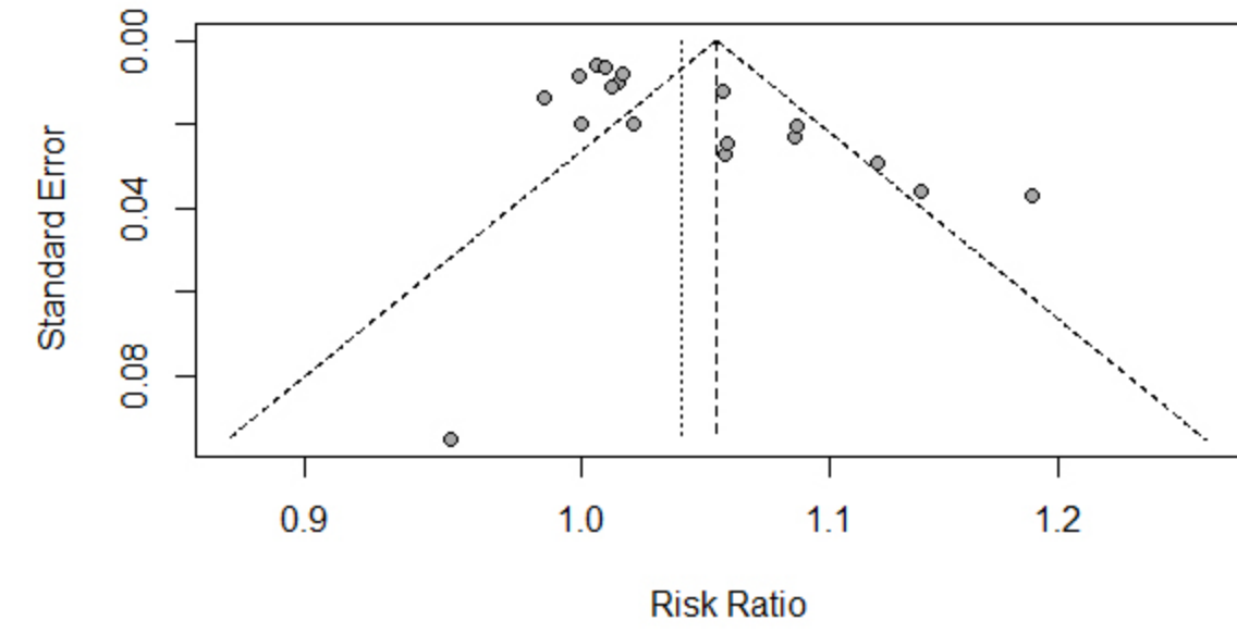
Screw position grade A+B funnel plot
