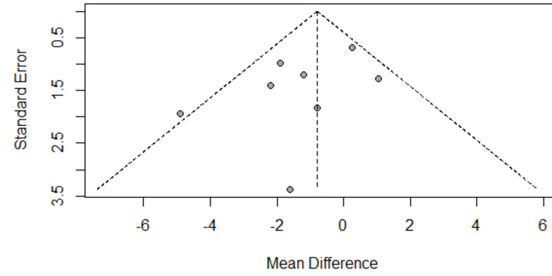
ODI scores funnel plot
