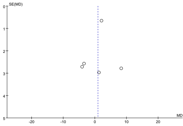
Lumbar lordosis funnel plot
