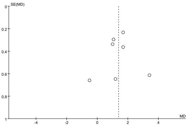
Intervertebral height funnel plot
