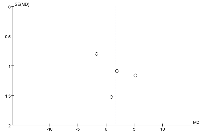
Fused segment lordosis funnel plot
