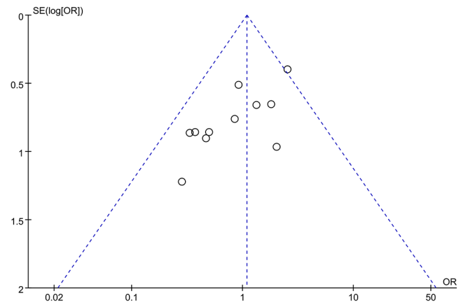
Complication funnel plot
