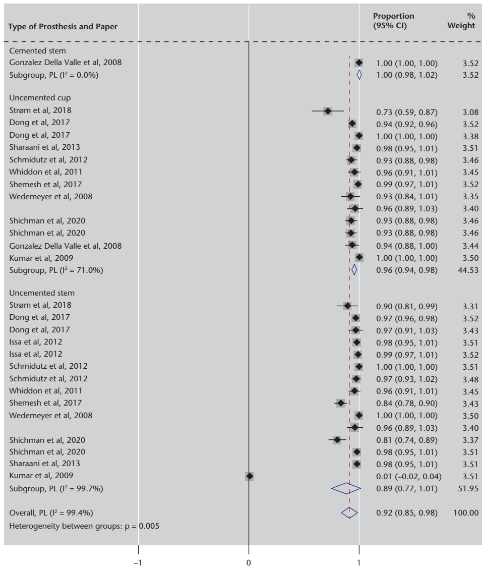
Fig. 4 Forest plot for two-size difference accuracy (±2) meta-analysis results.
