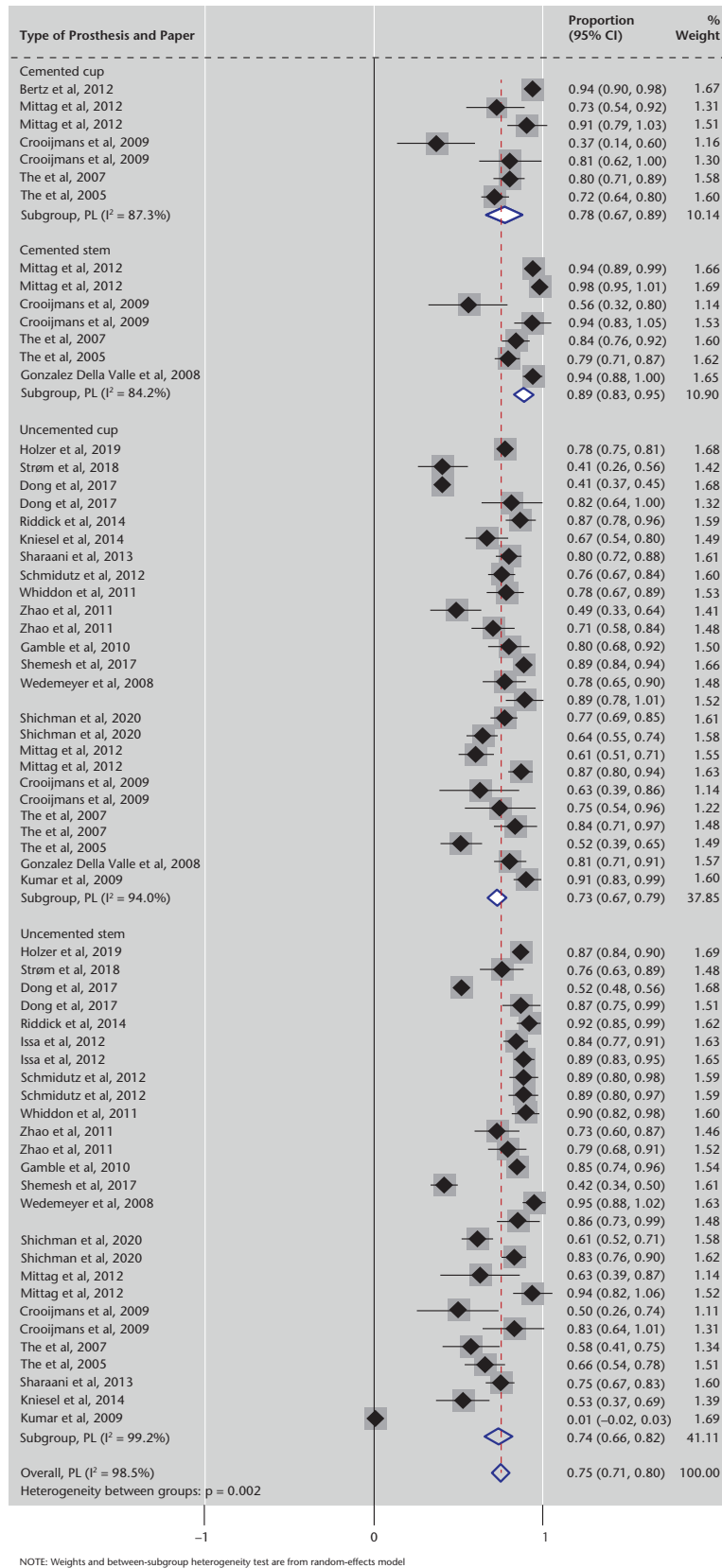
Fig. 3 Forest plot for one-size difference ( \pm 1 ) accuracy meta-analysis results.
